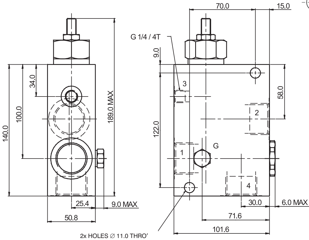
2x HOLES Ø 11.0 THRO'
